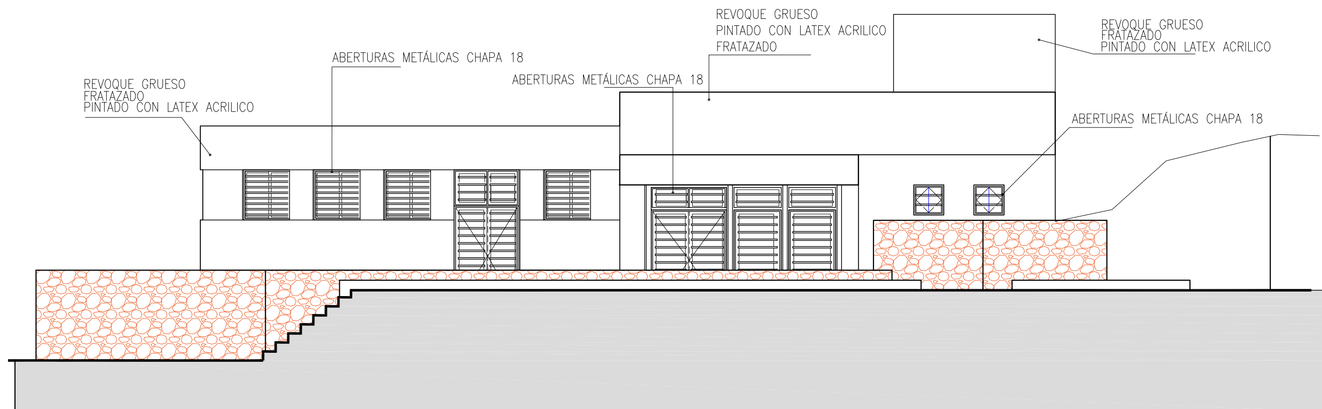
VISTA PRINCIPAL
